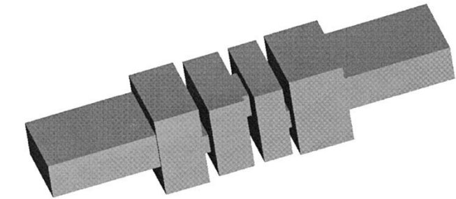
Fig. 1. Novel TM_{110} -mode inline filter structure utilizing bypass couplings of nonresonating TE_{10/01} modes.
