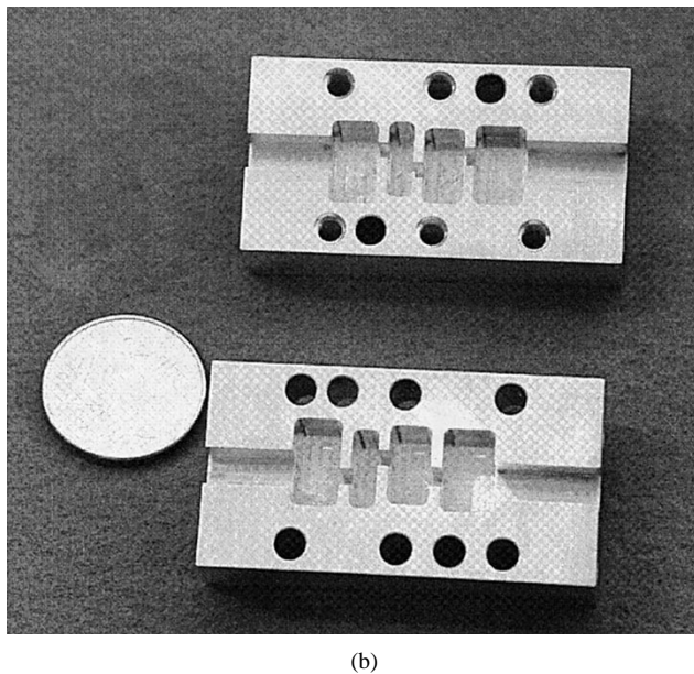
Fig. 9. (a) Comparison between computed and measured response of an inline four-pole TM_{110} -mode filter with two transmission zeros below and two above the passband. (b) Photograph of the two halves of the K -band prototype and size comparison with a 1-Euro-cent coin.
