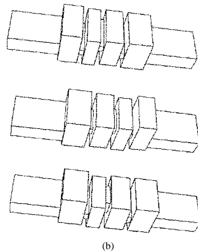
Fig. 8. (a) Responses of an inline four-pole TM_{110} -mode filter with four transmission zeros. (b) Filter arrangements with only capacitive irises (top), only inductive irises (middle), two capacitive, and a center inductive iris (bottom).
